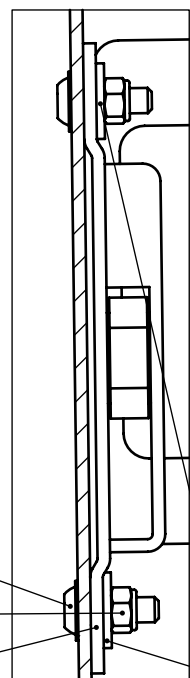
Section View I-I
