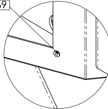
DETAIL D SCALE 1 : 3
