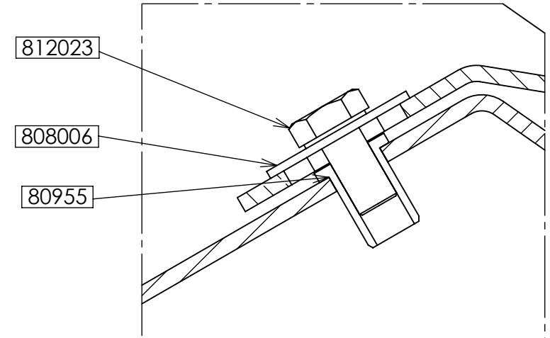
SECTION H-H SCALE 1 : 1
