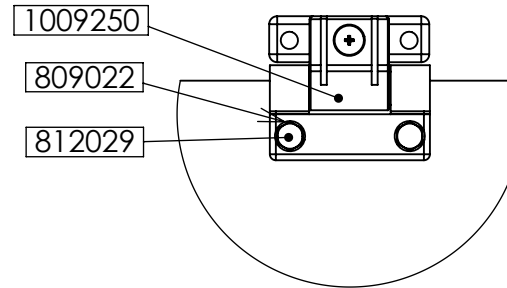
DETAIL L SCALE 1 : 3
