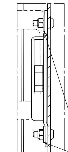
SECTION C-C SCALE 1 : 2
